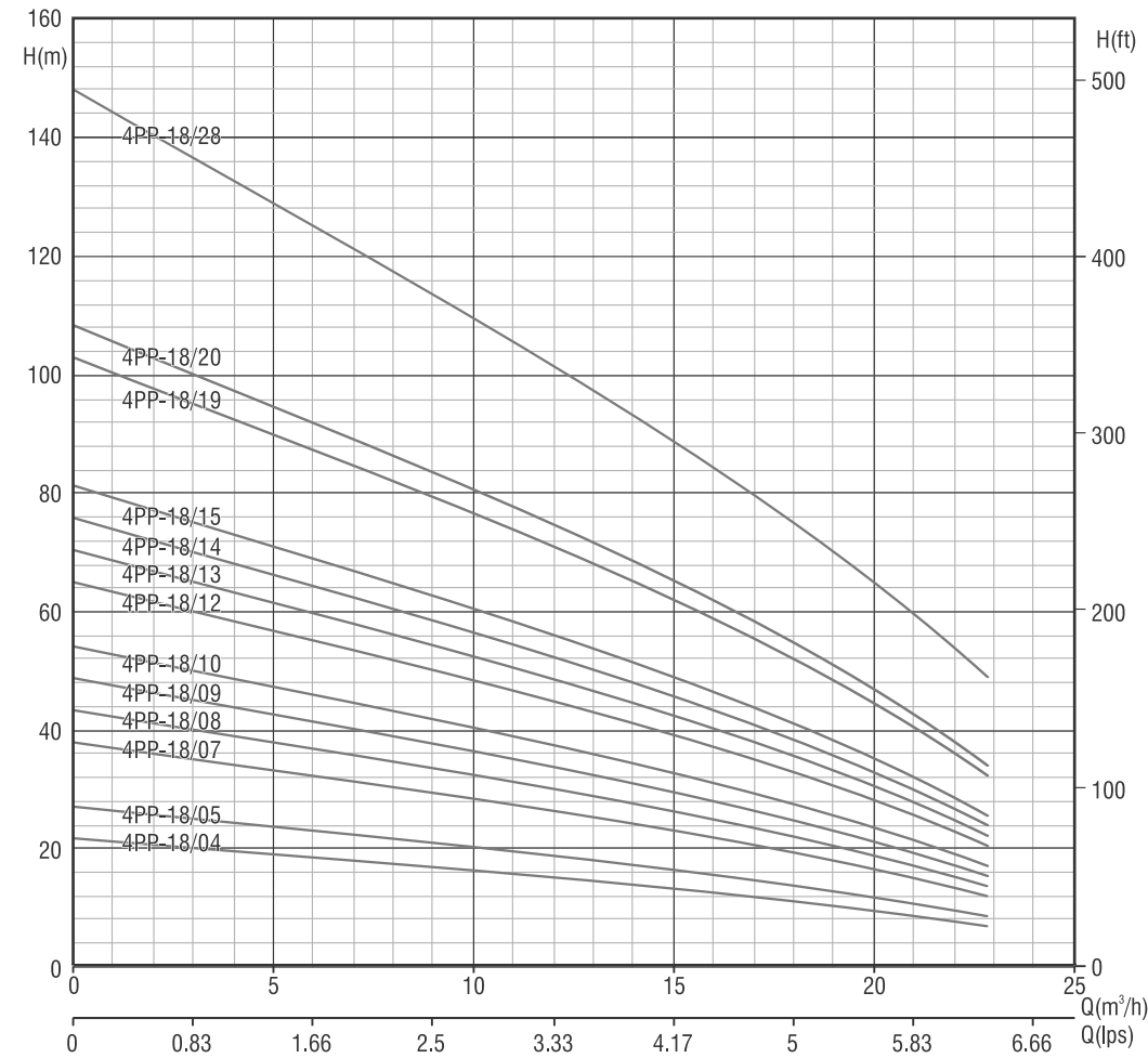
Performance Curve
