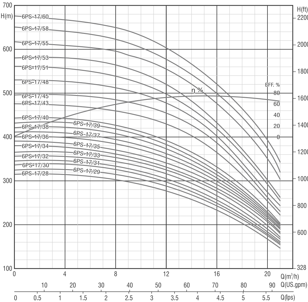
Performance Curve
