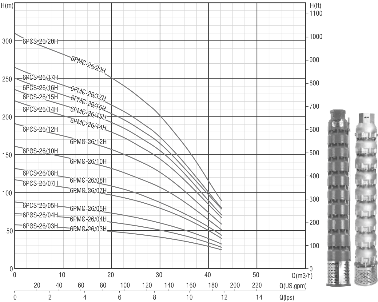
Performance Curve
