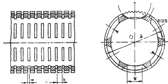
Ribbed Screen Pipe
